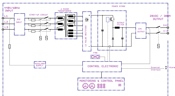
Block Diagram AC/DC Converter
