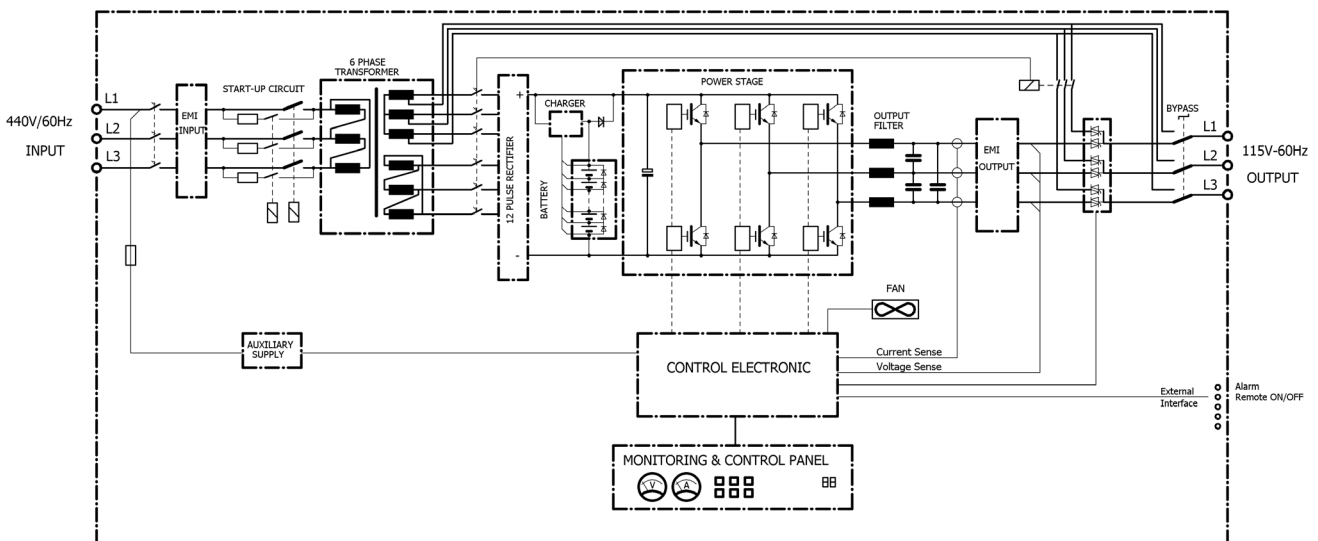
Converter / UPS System block diagram
